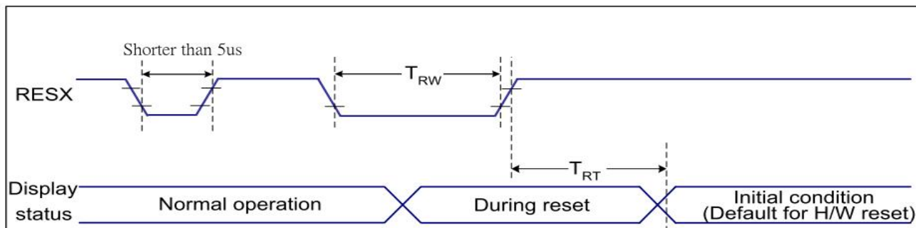
Reset Timing Characteristics IOVCC=1.65~1.95v Ta=25℃
